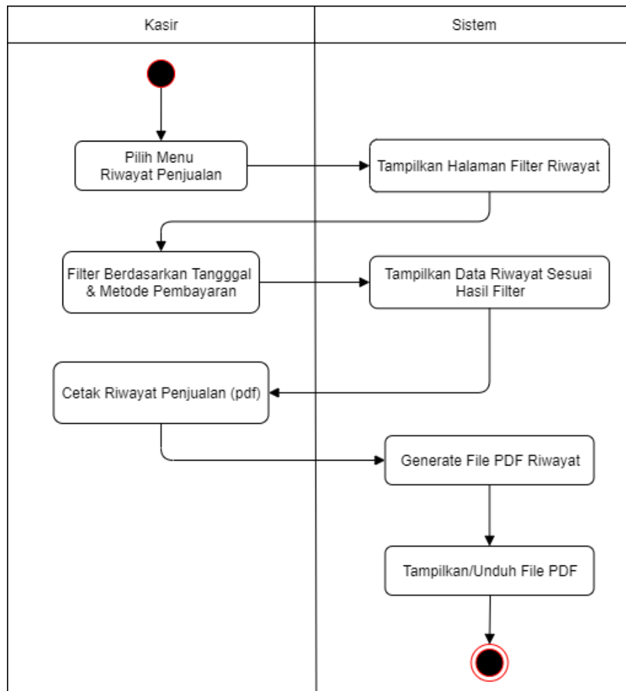
Gambar 5. Riwayat
